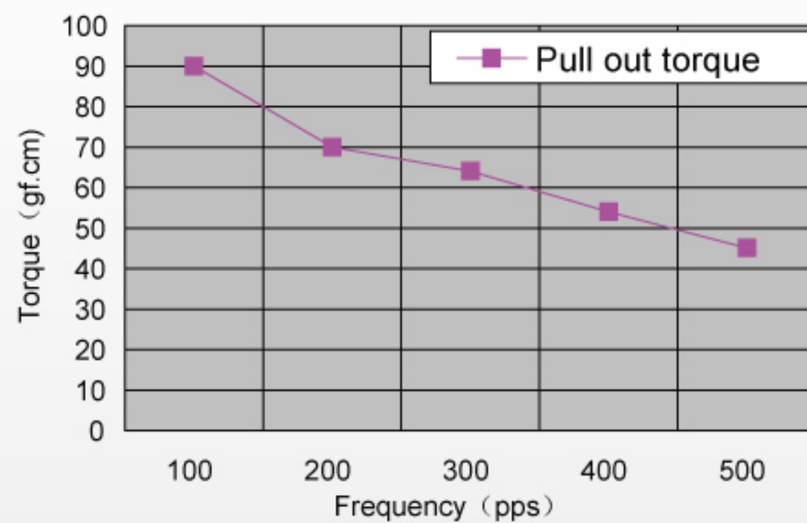
25BY46L BIPOLAR CHOPPER(at12[V],30[Ω])
