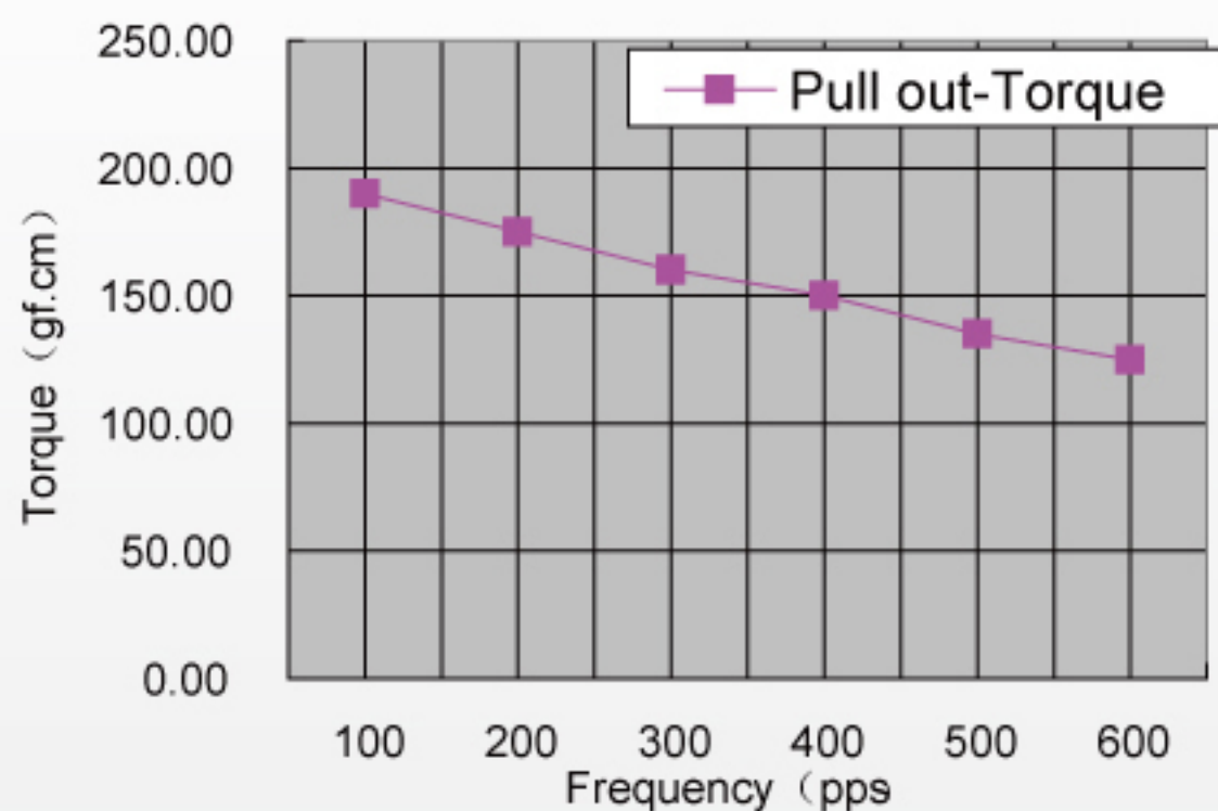
25BY46L UNIPOLAR CONST.VOLT(at24[V],50[Ω])
