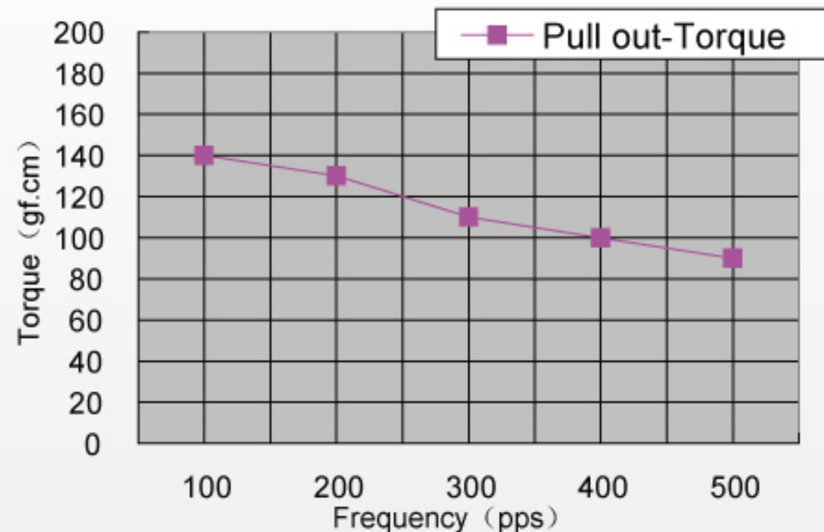
25BY412L UNIPOLAR CONST.VOLT(at20[V],90[Ω])
