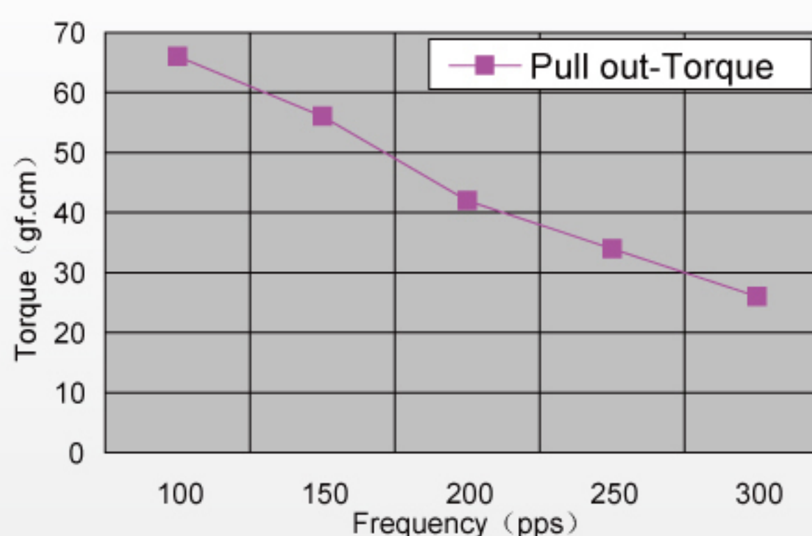
25BY412L BIPOLAR CHOPPER(at5[V],50[Ω])
