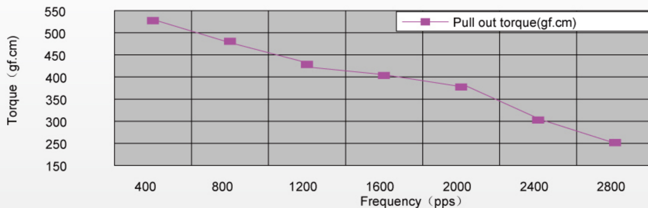
42BY412S BIPOLAR CHOPPER(at24[V],16[Ω],400[mA])
